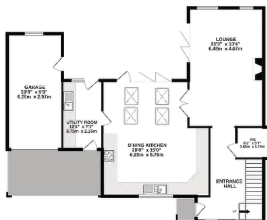
GROUND FLOOR 1105 sq.ft. (102.6 sq.m.) approx.
